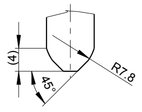
DETAIL EXTREMITE TRINGLE INFERIEURE
